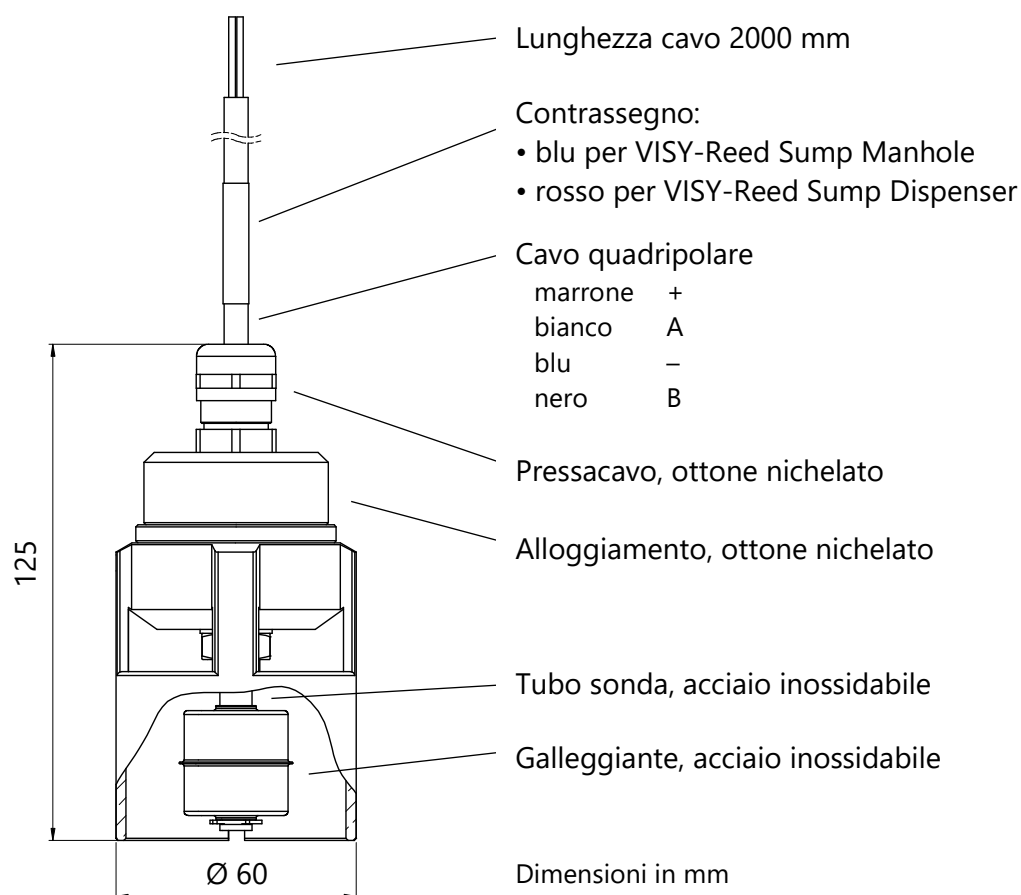
Figura 12: VISY-Reed Sump
