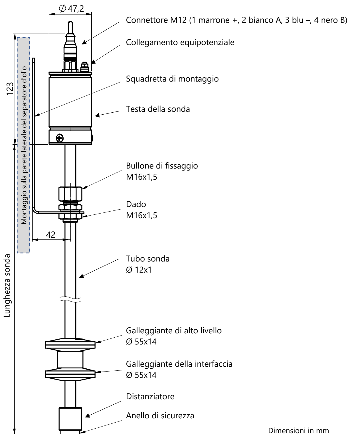
Figura 13: VISY-Stick Oil
