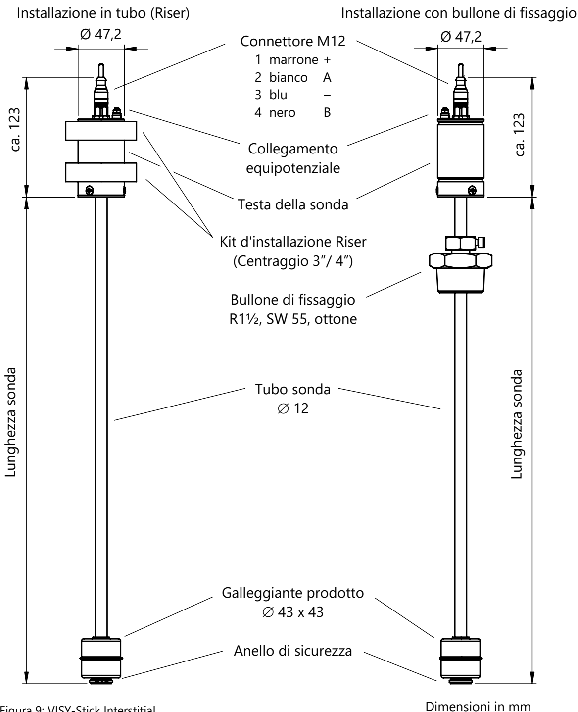
Figura 9: VISY-Stick Interstitial
