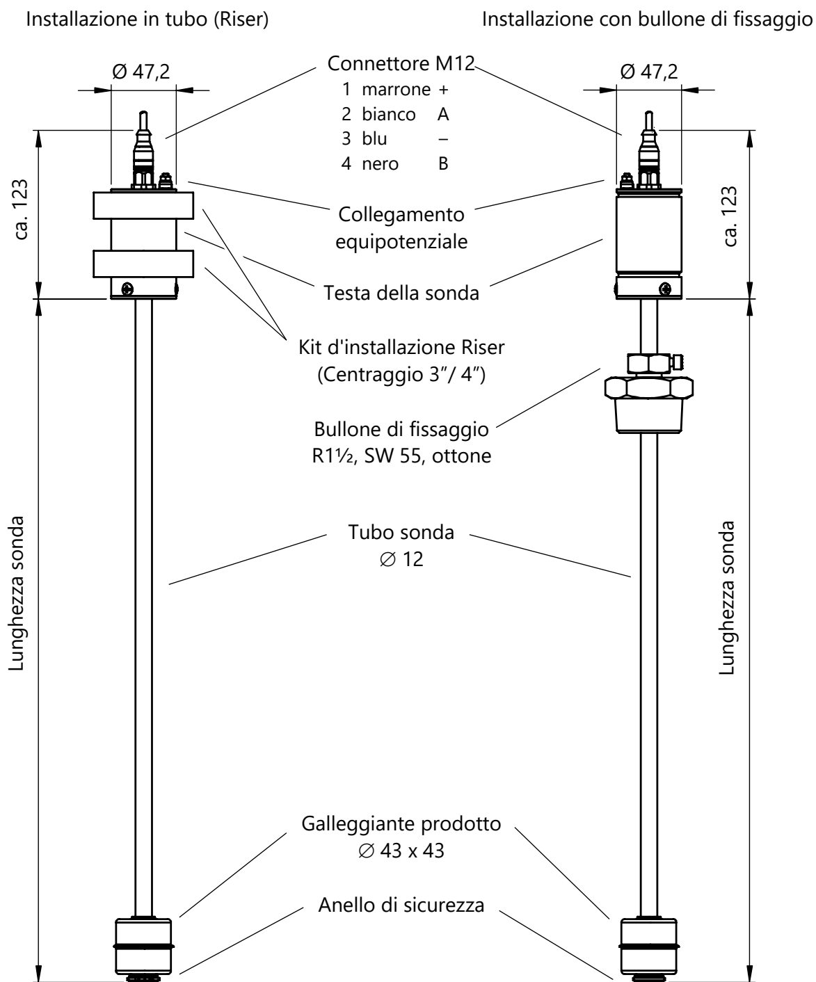
Figura 4: VISY-Stick Ethanol
