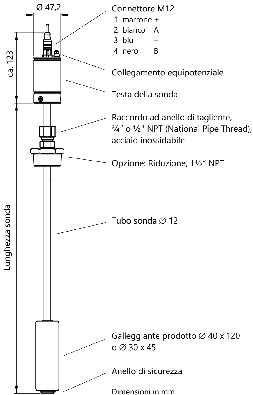
Figura 8: VISY-Stick LPG
