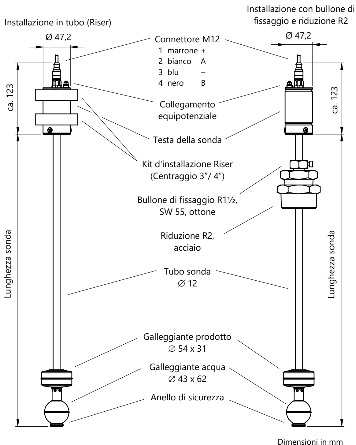
Figura 3: VISY-Stick Advanced
