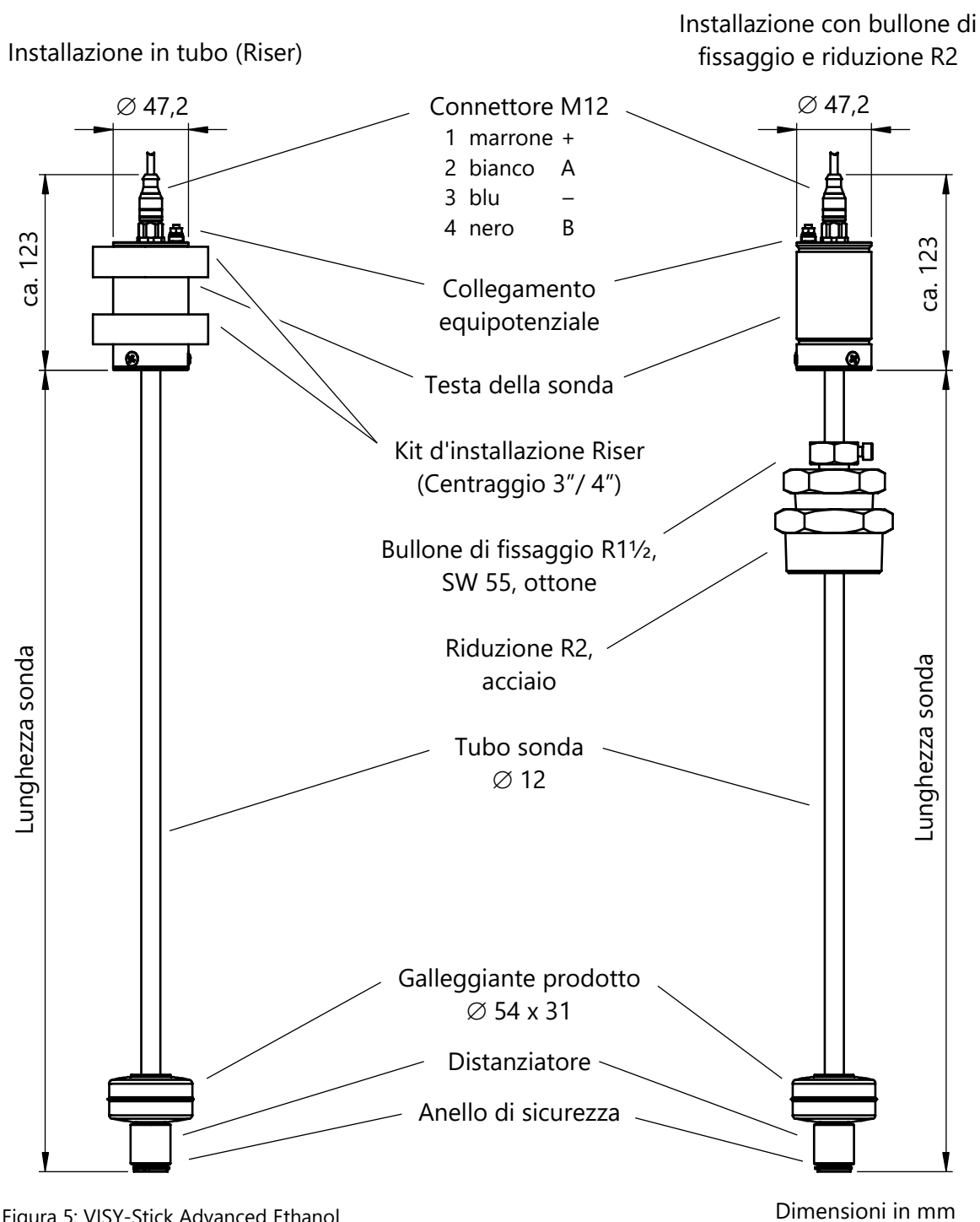
Figura 5: VISY-Stick Advanced Ethanol
