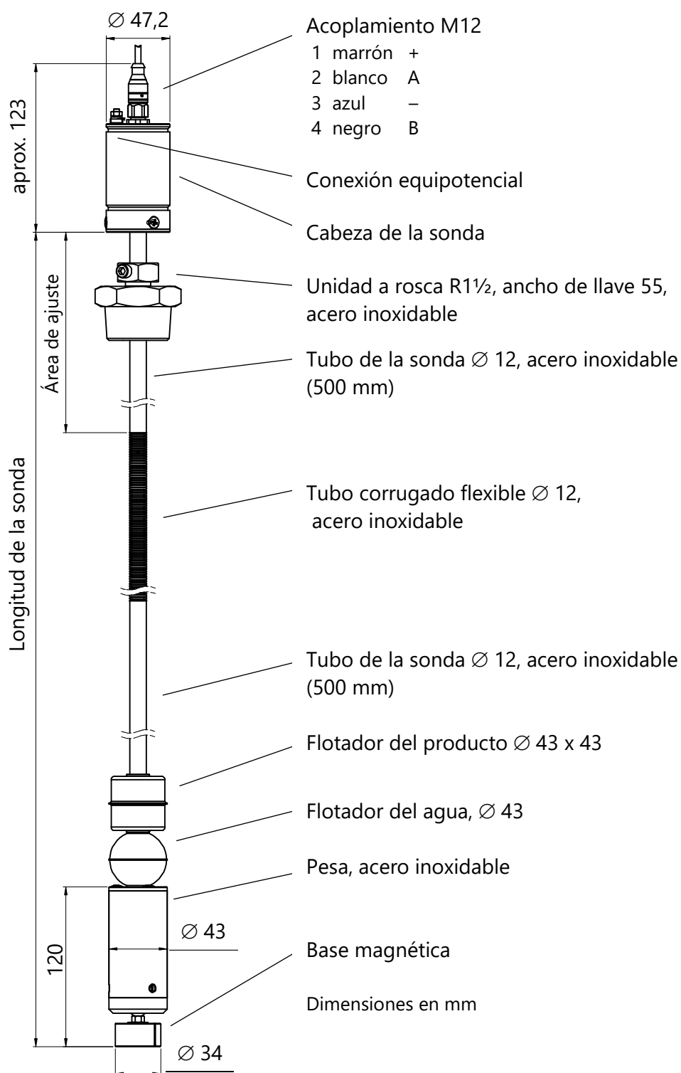
Figura 7: VISY-Stick Flex
