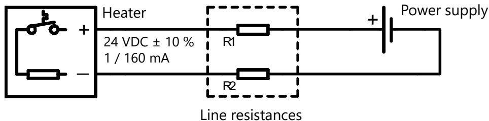
Figure 10: Wiring diagram TORRIX (Exd) XTSH heater
