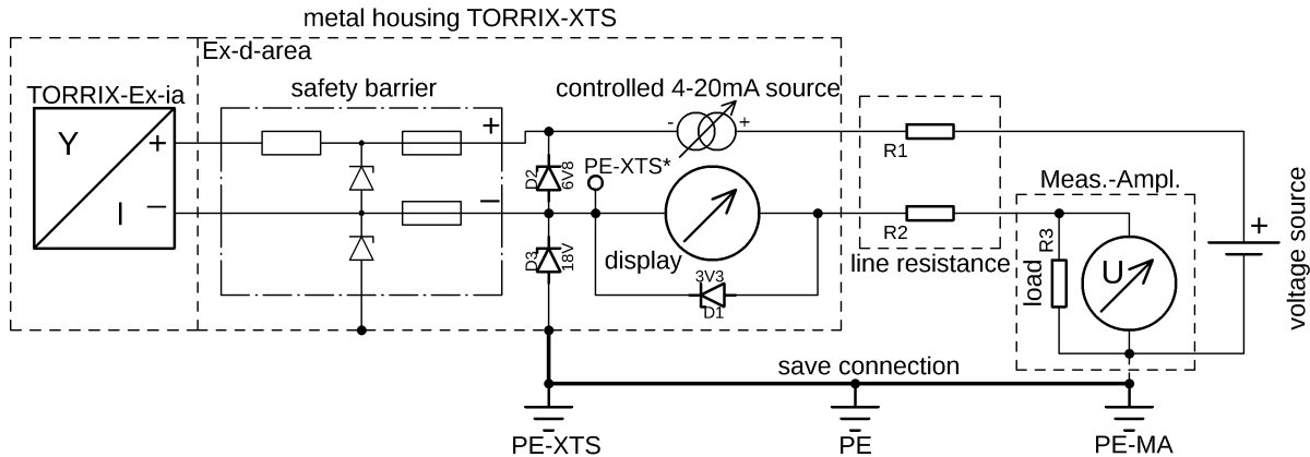
Figure 9: Wiring diagram TORRIX Exd XTS
