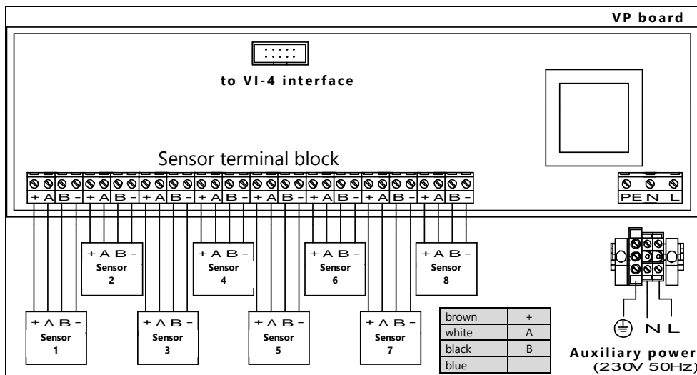
Figure 1: VISY-Command 8 with one VP-1 board for 8 sensors
