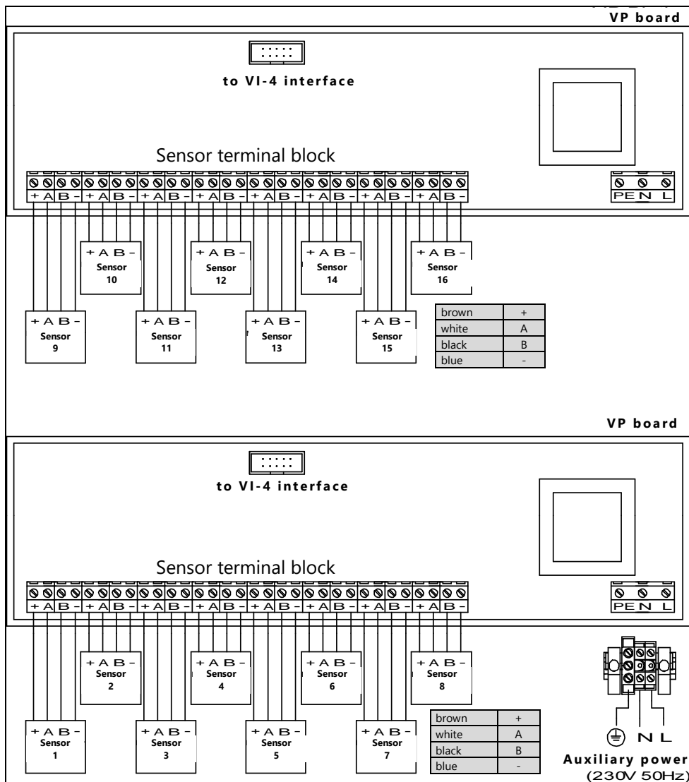
Figure 2: VISY-Command 16 with two VP-1 boards for 16 sensors
