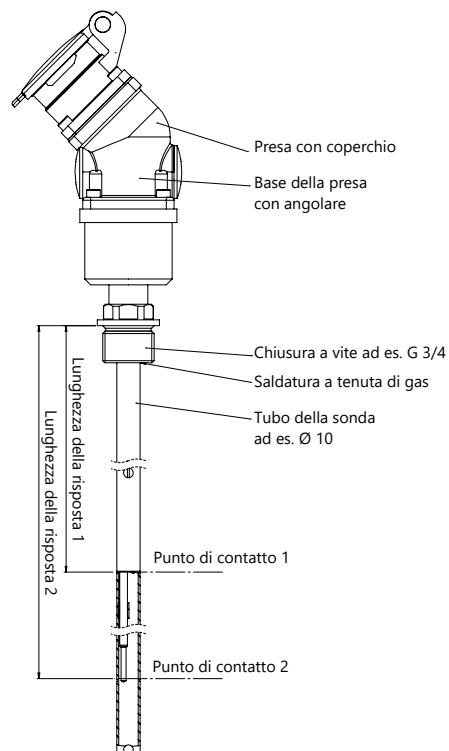
Figura 1.4d: LS 300 E Steck/01
