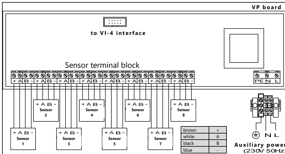
Figure 1: VISY-Command 8 with one VP-1 board for 8 sensors
