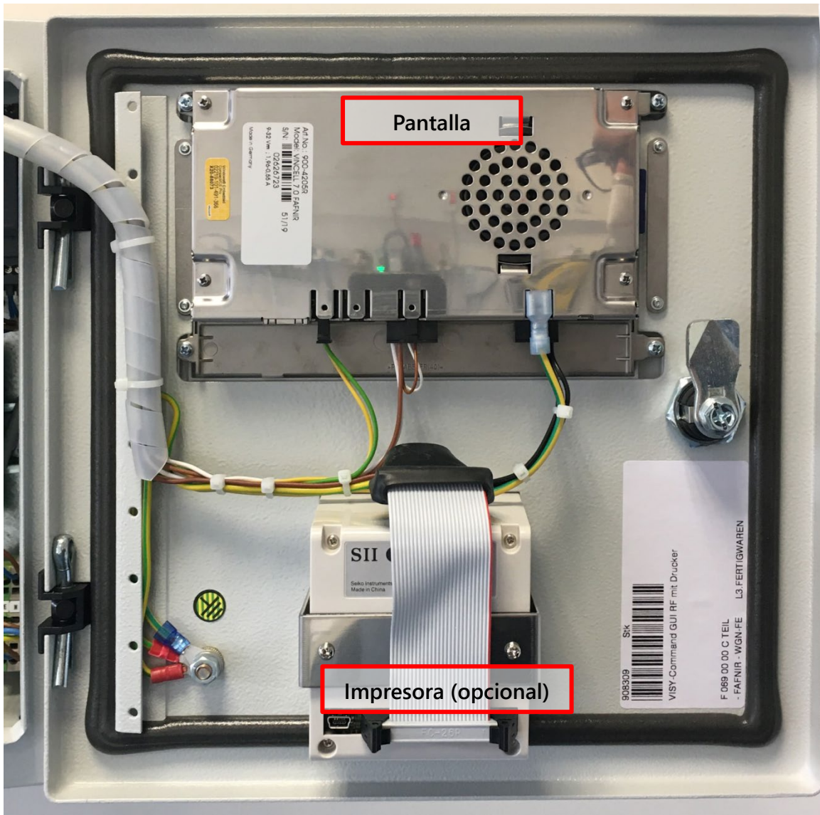
Figura 3: VISY-Command GUI tapa de carcasa, vista interior
