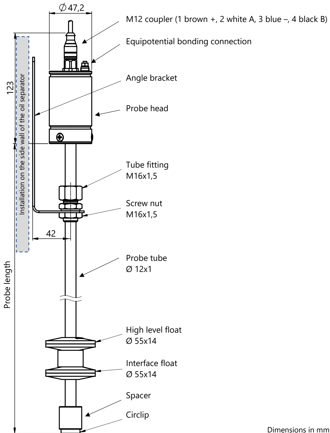
Figure 13: VISY-Stick Oil
