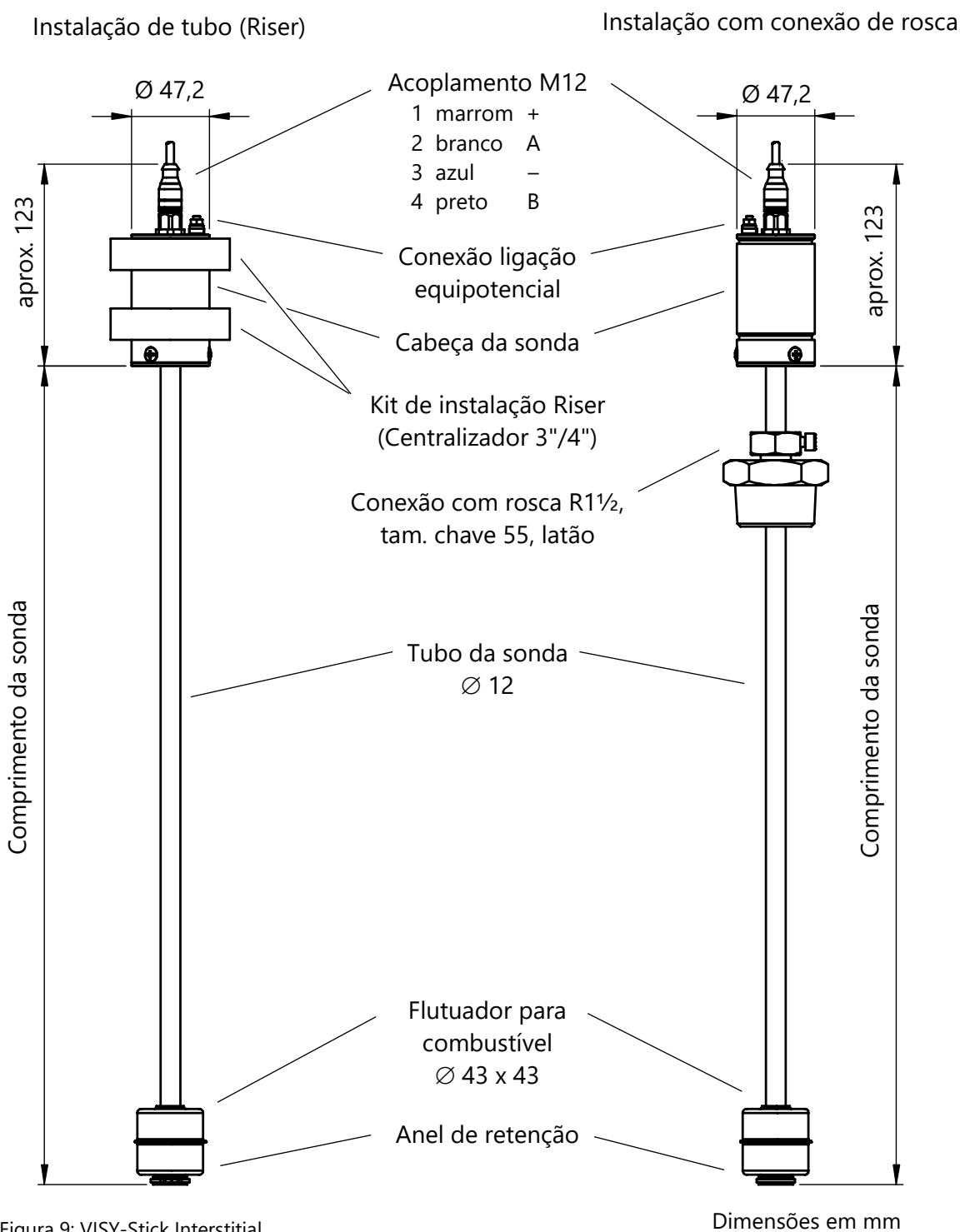
Figura 9: VISY-Stick Interstitial
