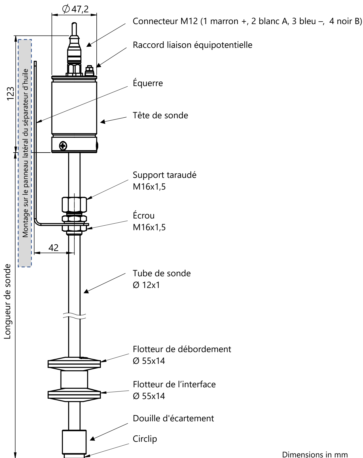
Figure 13 : VISY-Stick Oil
