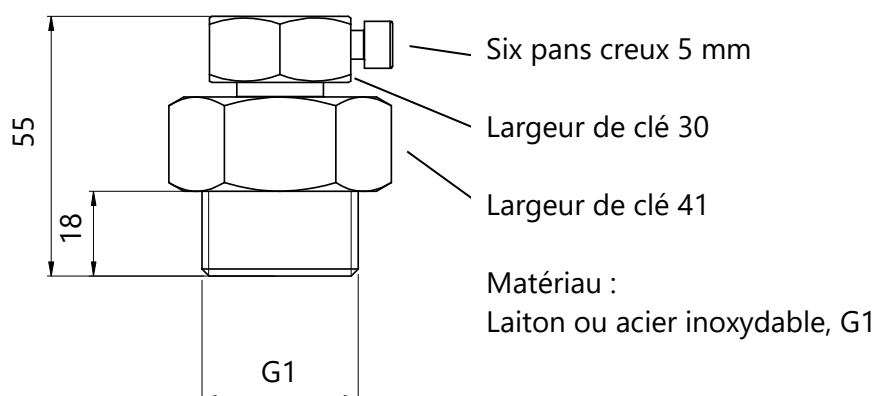
Figure 18 : Support taraudé 1"
