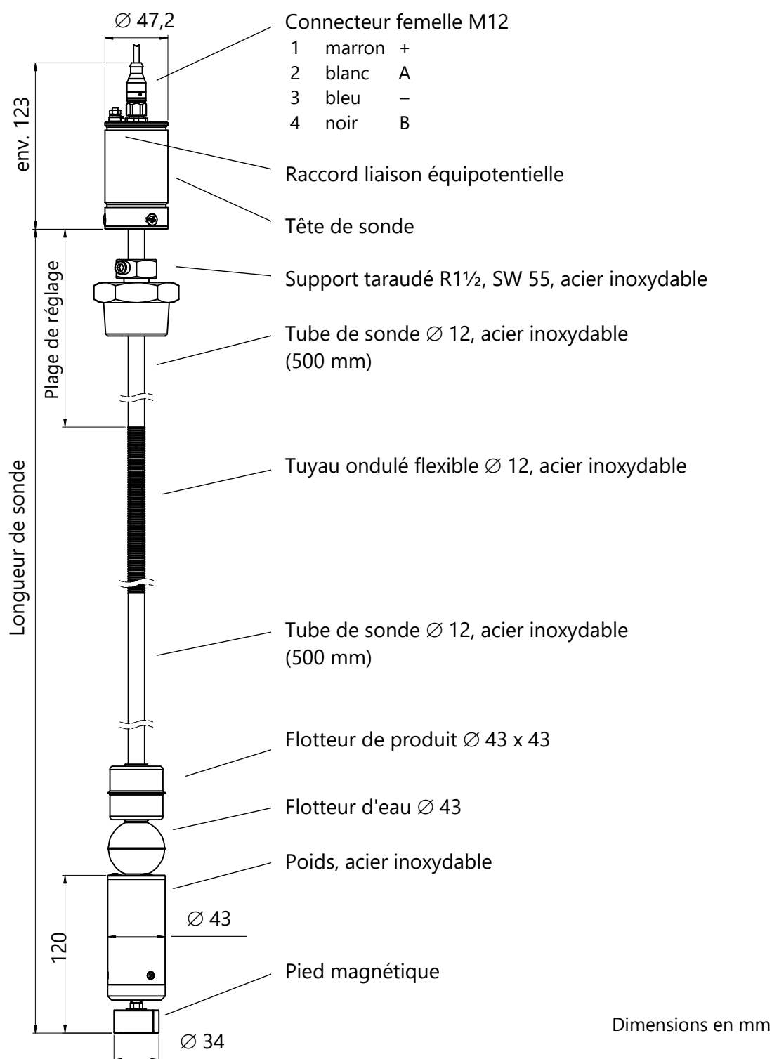
Figure 7 : VISY-Stick Flex
