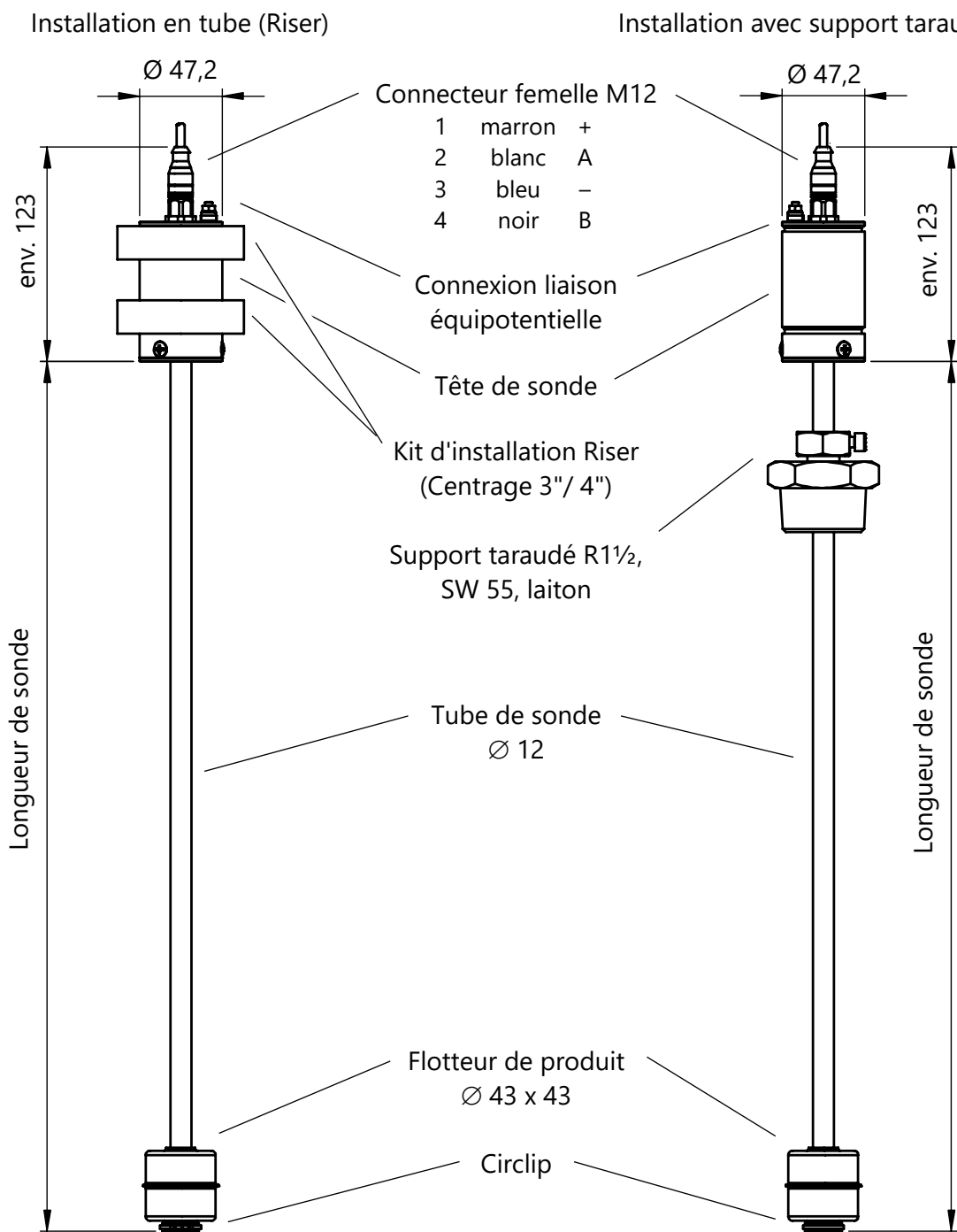
Figure 9 : VISY-Stick Interstitial
