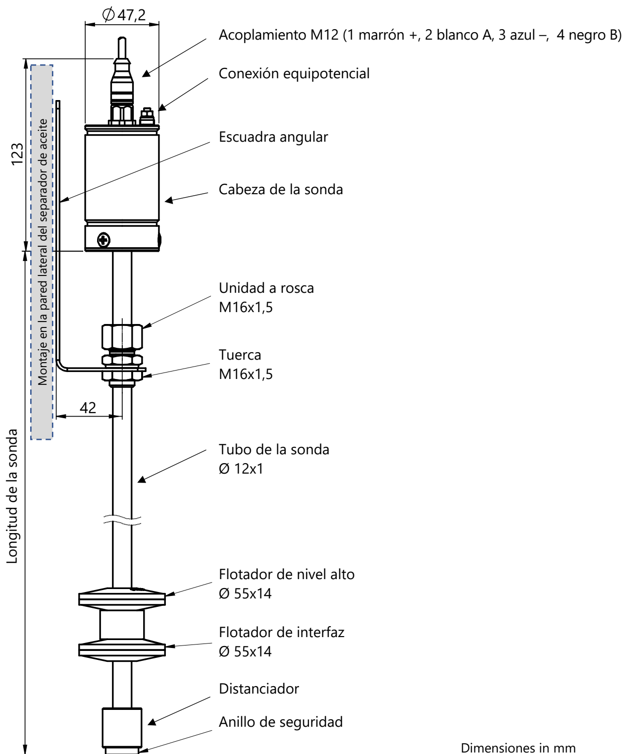
Figura 13: VISY-Stick Oil
