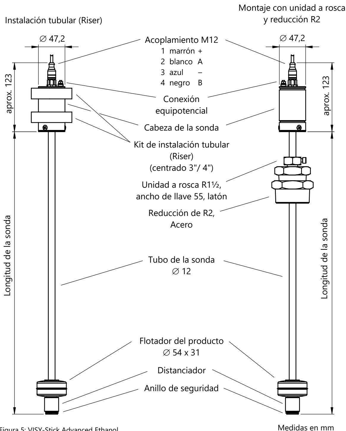
Figura 5: VISY-Stick Advanced Ethanol
