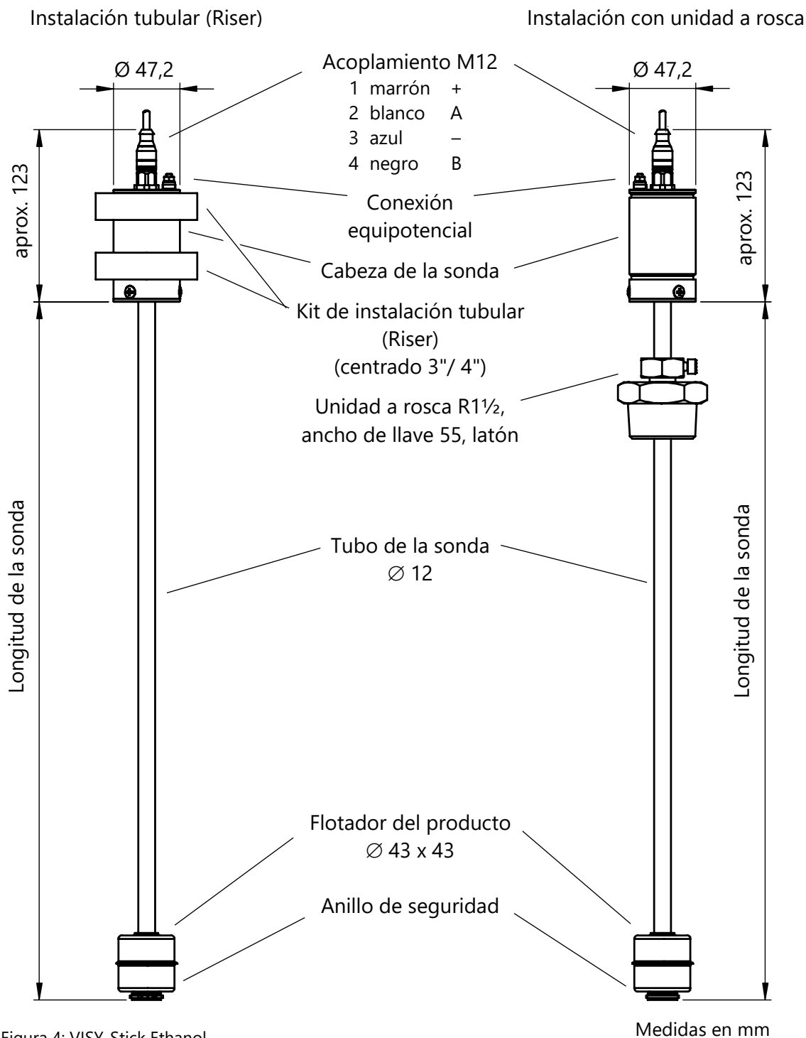
Figura 4: VISY-Stick Ethanol
