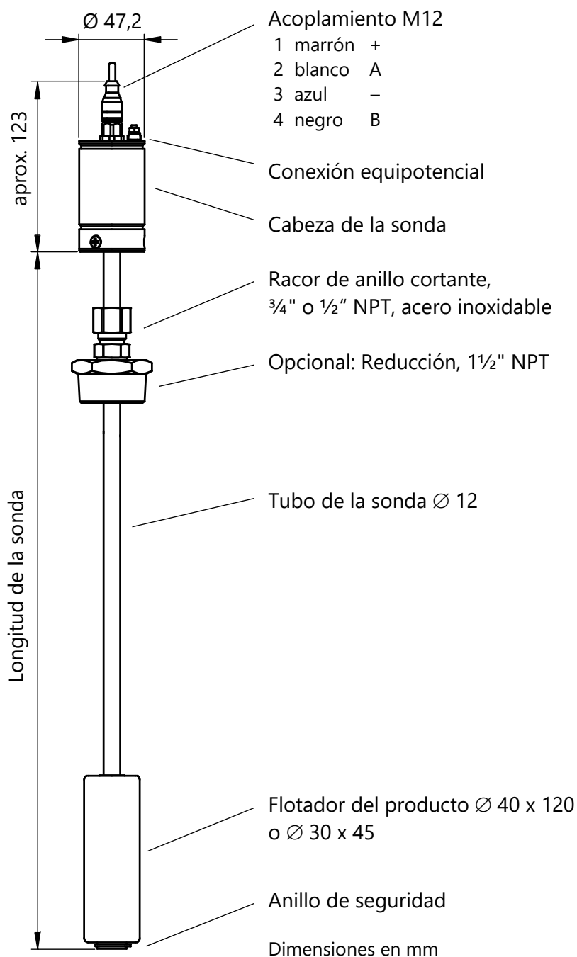
Figura 8: VISY-Stick LPG
