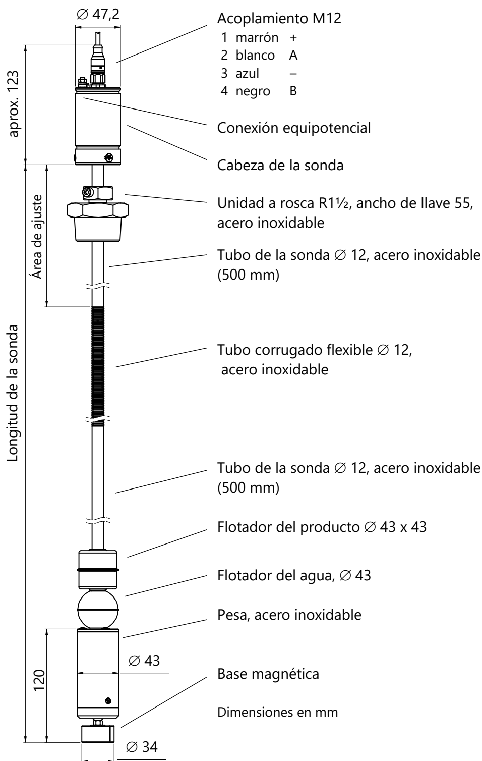
Figura 7: VISY-Stick Flex
