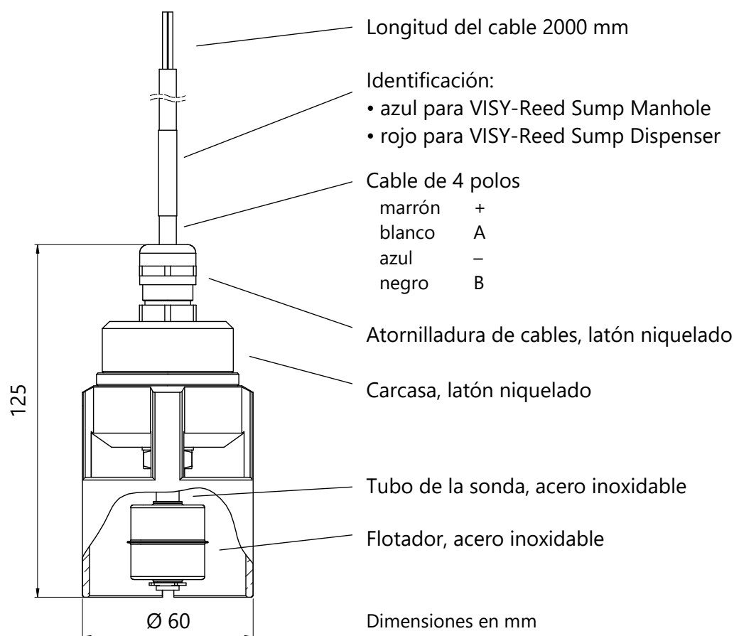
Figura 12: VISY-Reed Sump
