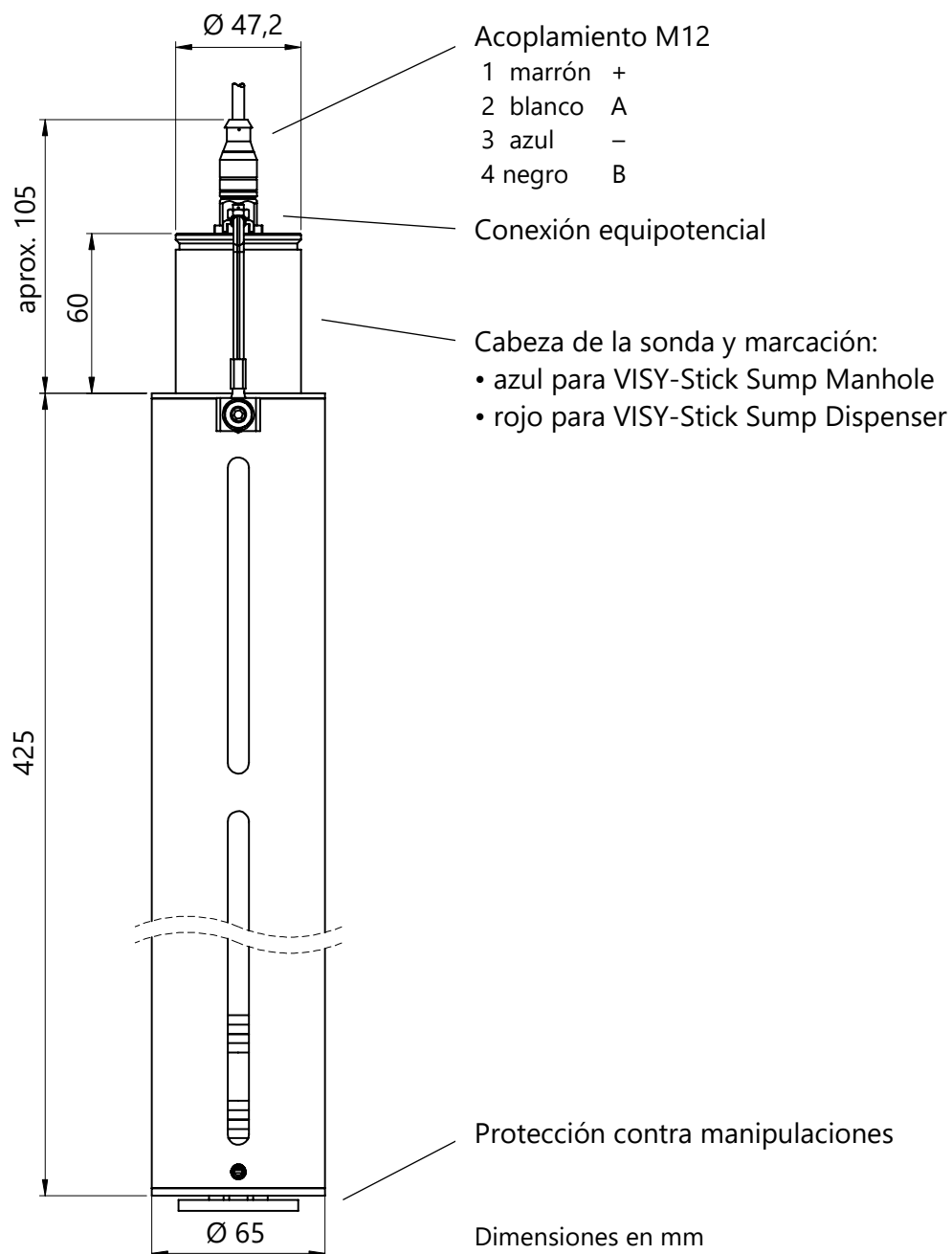
Figura 11: VISY-Stick Sump
