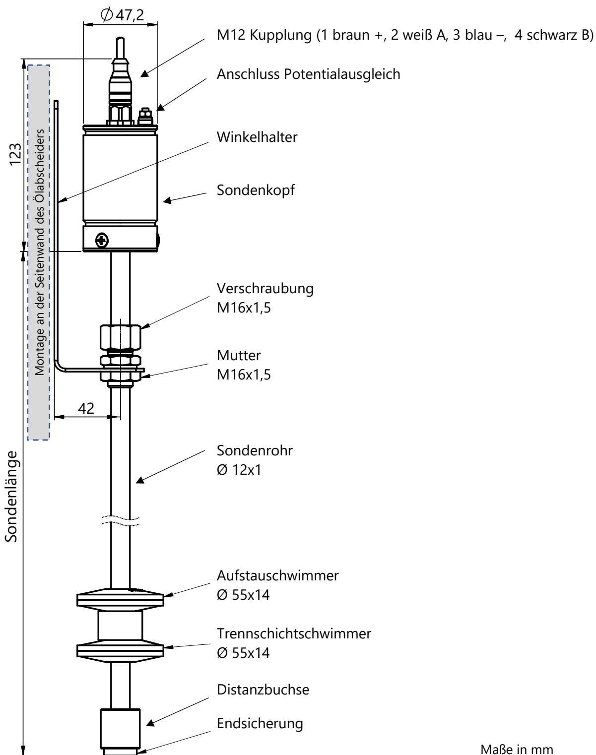
Abbildung 13: VISY-Stick Oil
