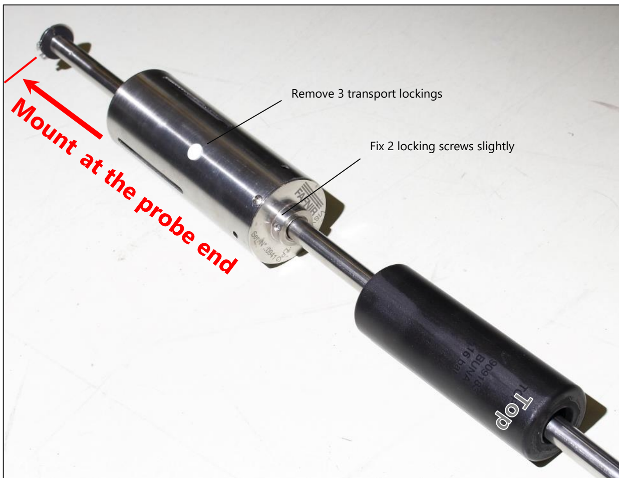
Figure 5: Accessories mounting
