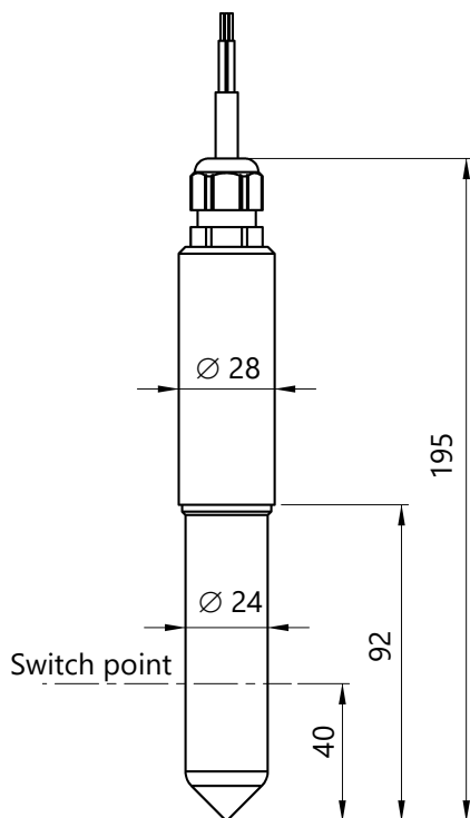
Figure 1: SEPARIX-C L Plus, dimensions
