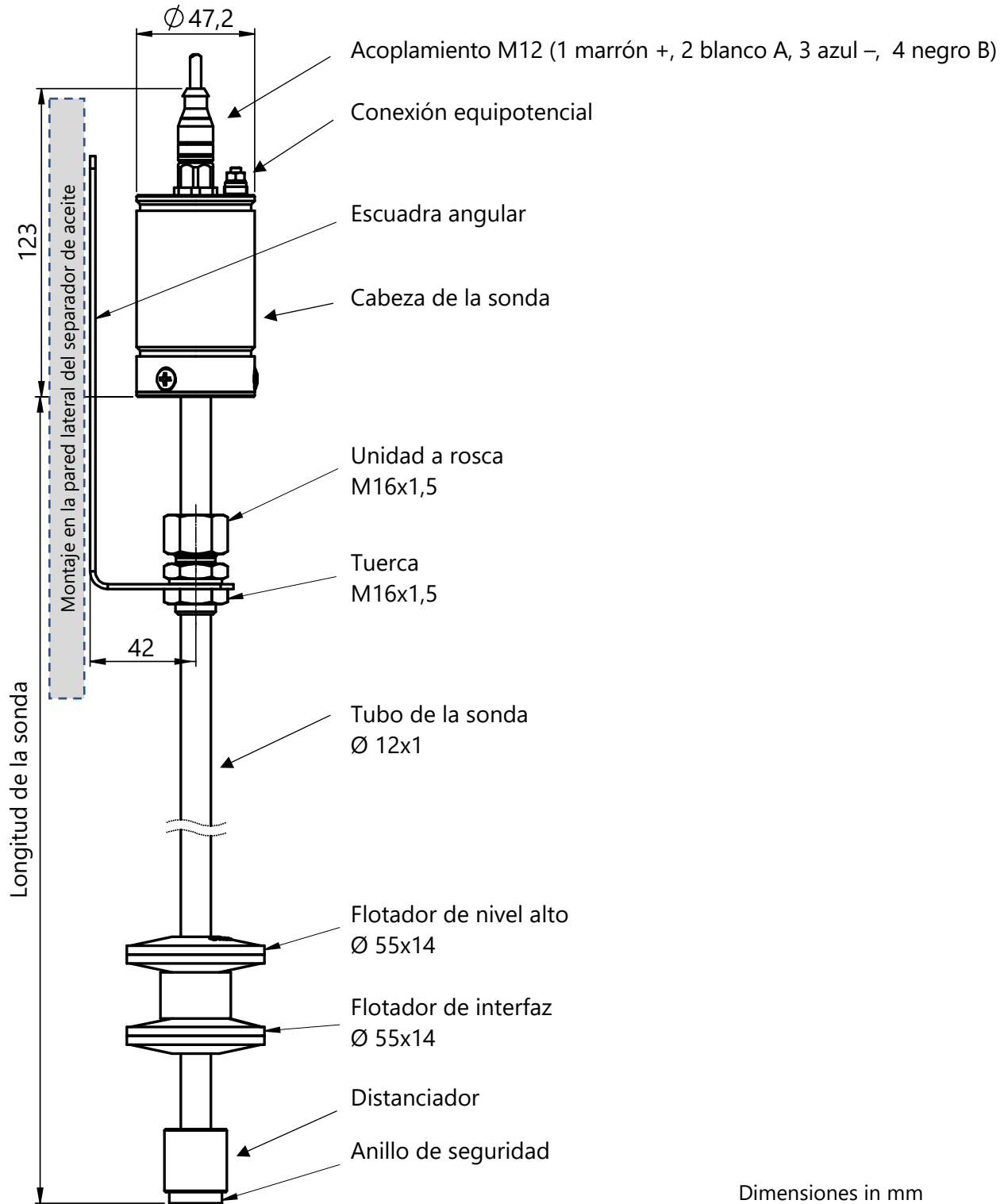
Figura 13: VISY-Stick Oil
