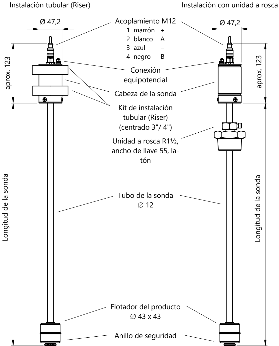
Figura 9: VISY-Stick Interstitial
