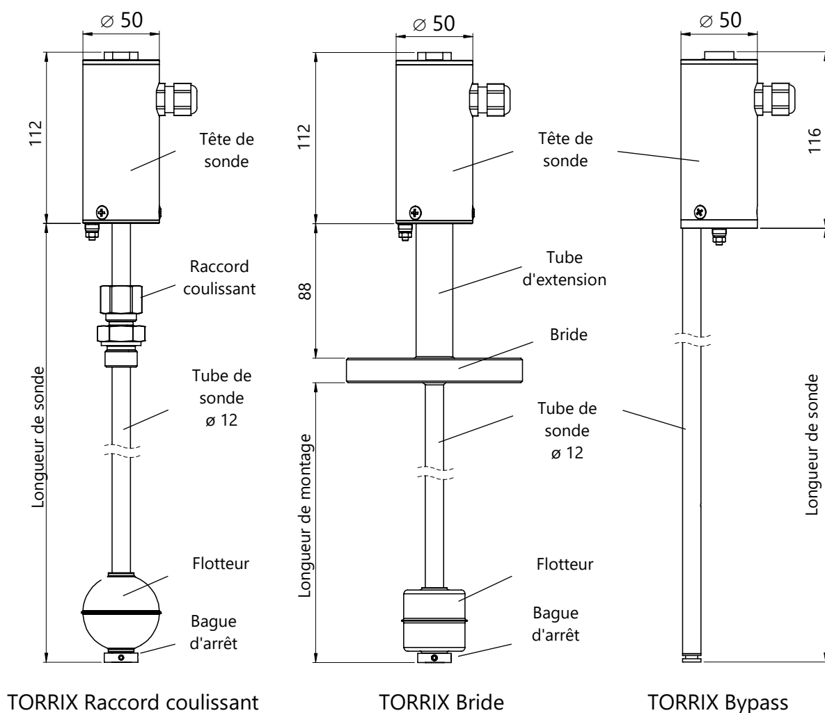
Figure 3 : Versions TORRIX
