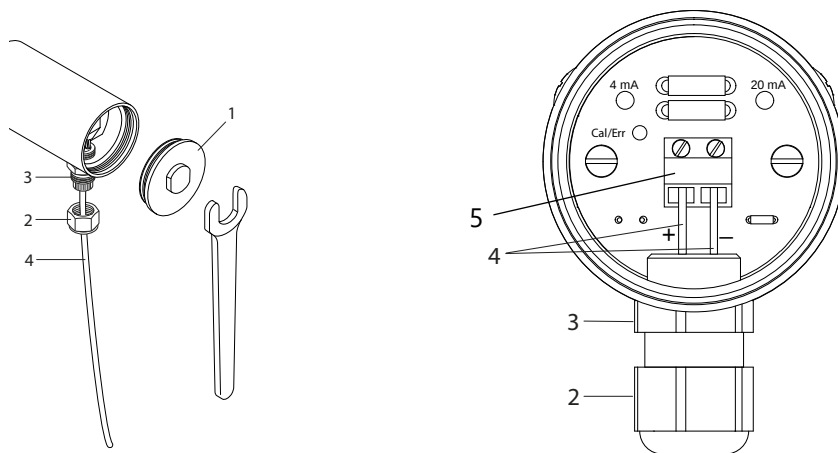
Figure 9 : Câblage
