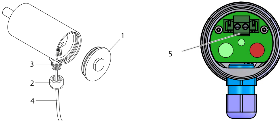
Figure 9 : Câblage
